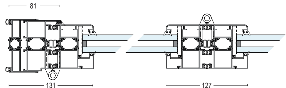
Folding sliding doors. Technical information.
