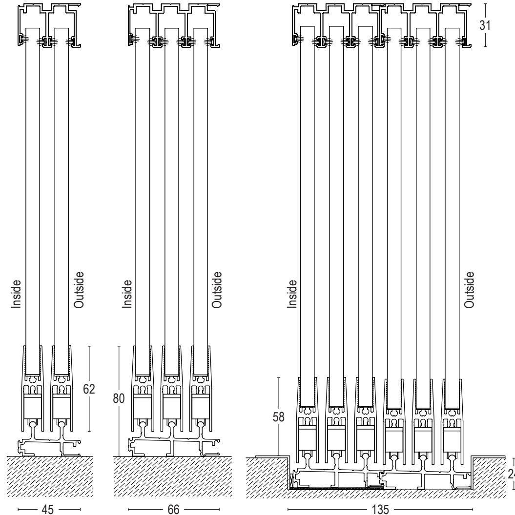
Surface-mounted two-track guide
