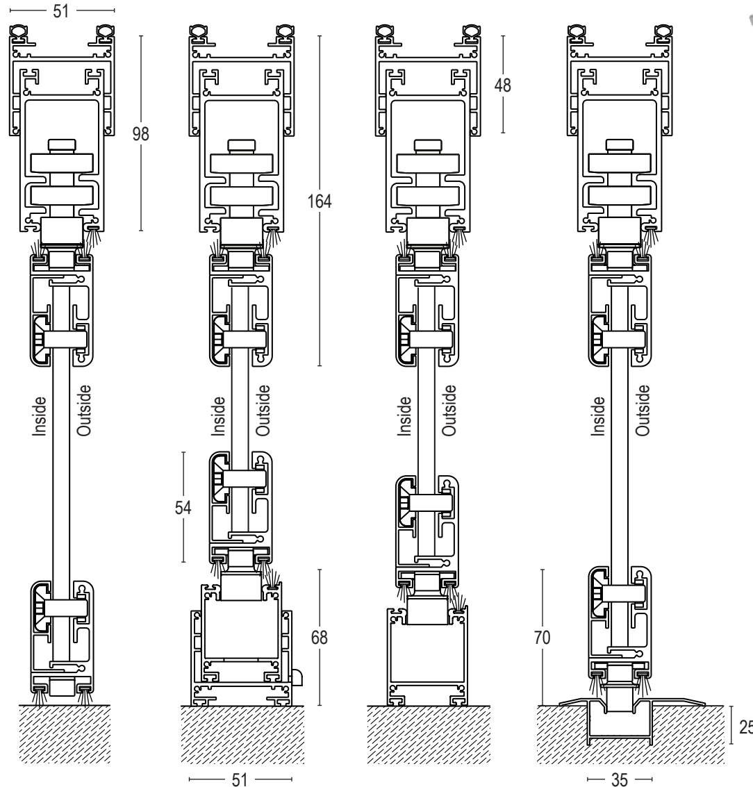
Without bottom track
